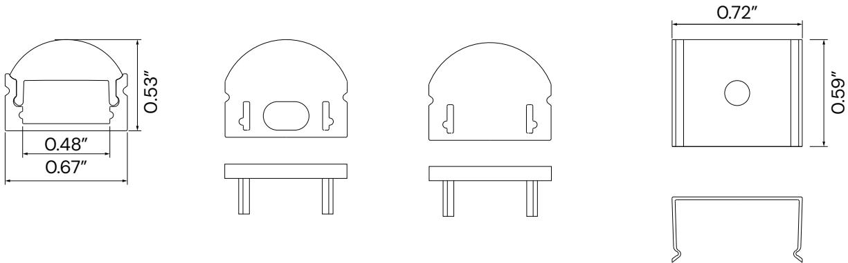
CROSS SECTION
