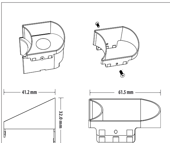
BASILISK-LOUVER (1 LOUVER NEEDED FOR EACH LINK)
