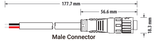
Male Connector
