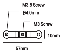
AA-MC-CLIP Fixed Bracket
