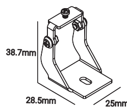
AA-PVT-CLIP Adjustable Bracket
